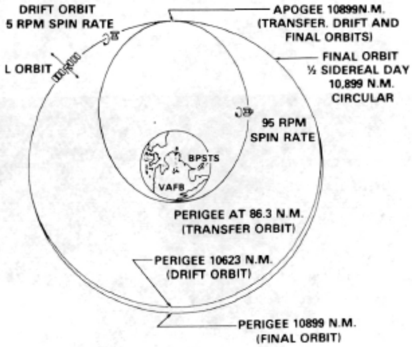
Fig. 3 - Mission sequence of NTS-2 events
