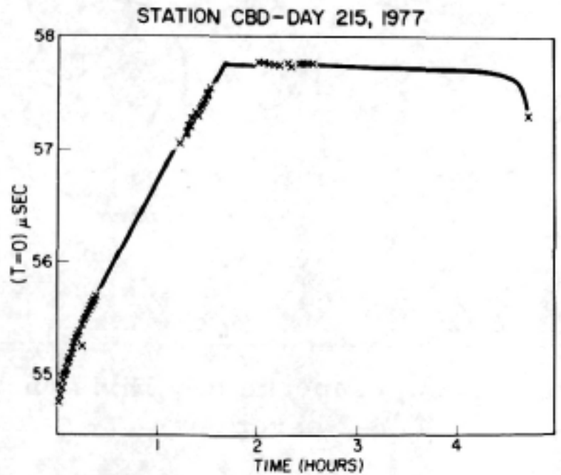
Fig. 21 - Effect of relativity correction
