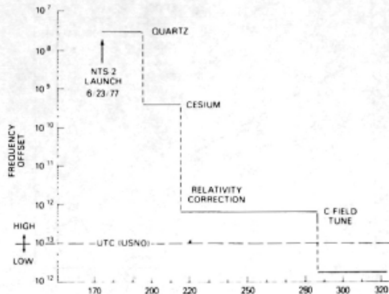
Fig. 27 - Frequency offset summary
