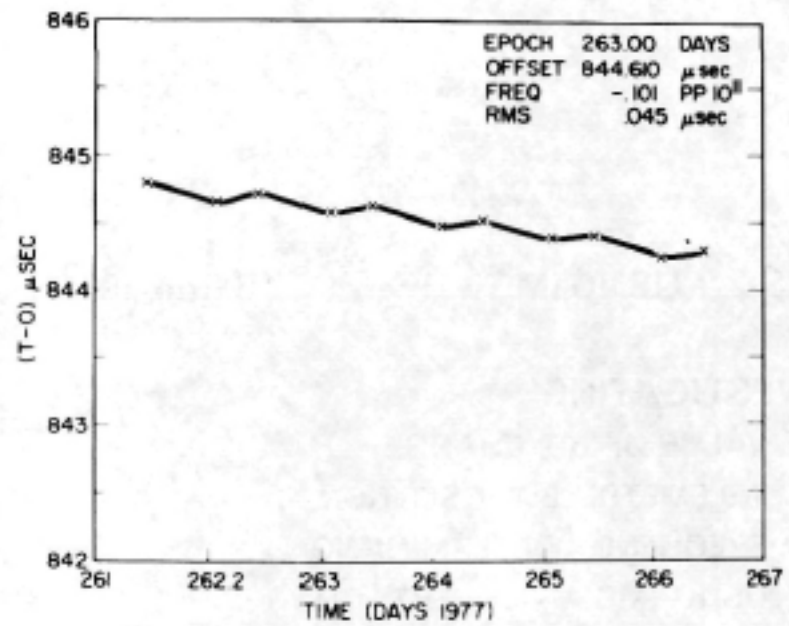
Fig. 23 - Frequency, NTS-CBD
