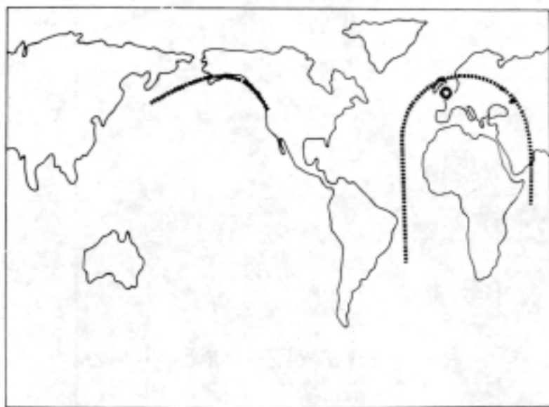
Fig. 14 - Royal Greenwich Observatory NTS-2 coverage
