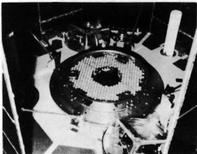
Fig. 34 - NTS-1 laser retroreflector
