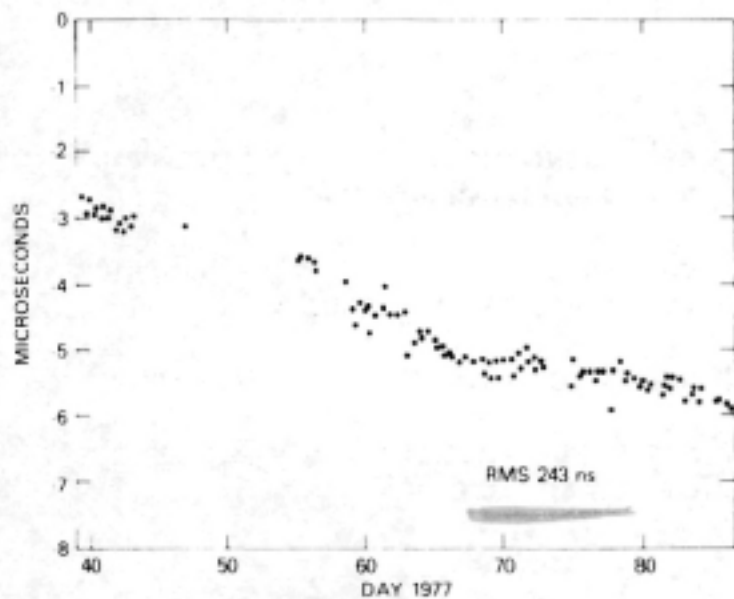
Fig. 29 - NTS-1 time transfer, NASA Cape Kennedy Station
