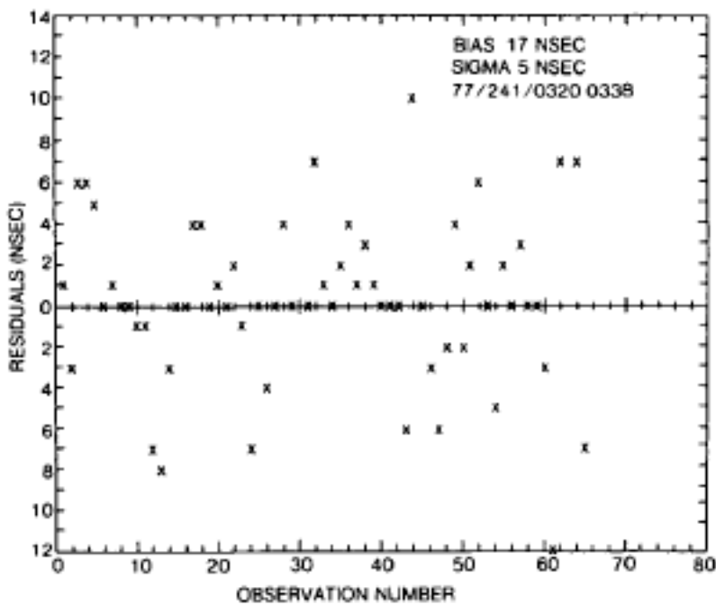
Fig. 40 - Laser returns, Mt. Hopkins, 1977 day 241
