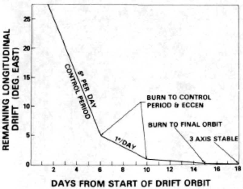
Fig. 8 - Pre-launch NTS-2 drift orbit profile
