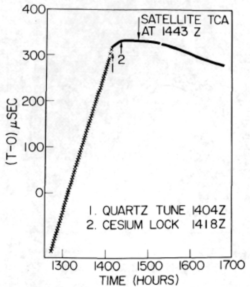
Fig. 19 - Cesium frequency standard lock up, 1977 day 190, 1418 UTC
