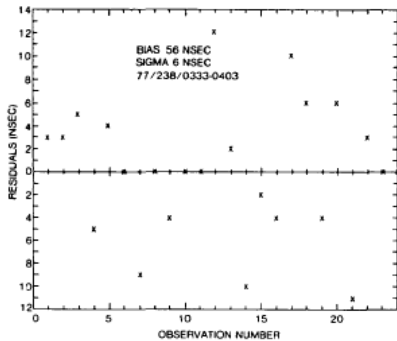
Fig. 39 - Laser residuals, Mt. Hopkins, 1977 day 238
