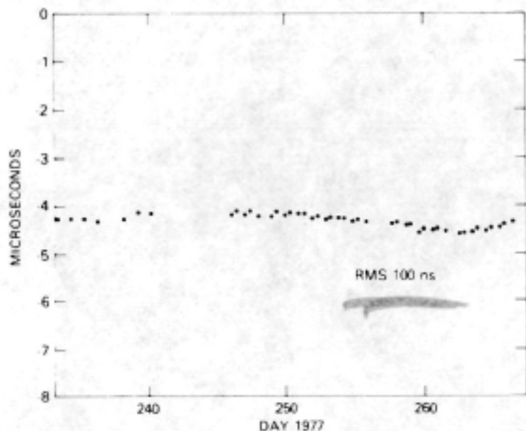
Fig. 30 - NTS-2 time transfer, NASA Cape Kennedy station
