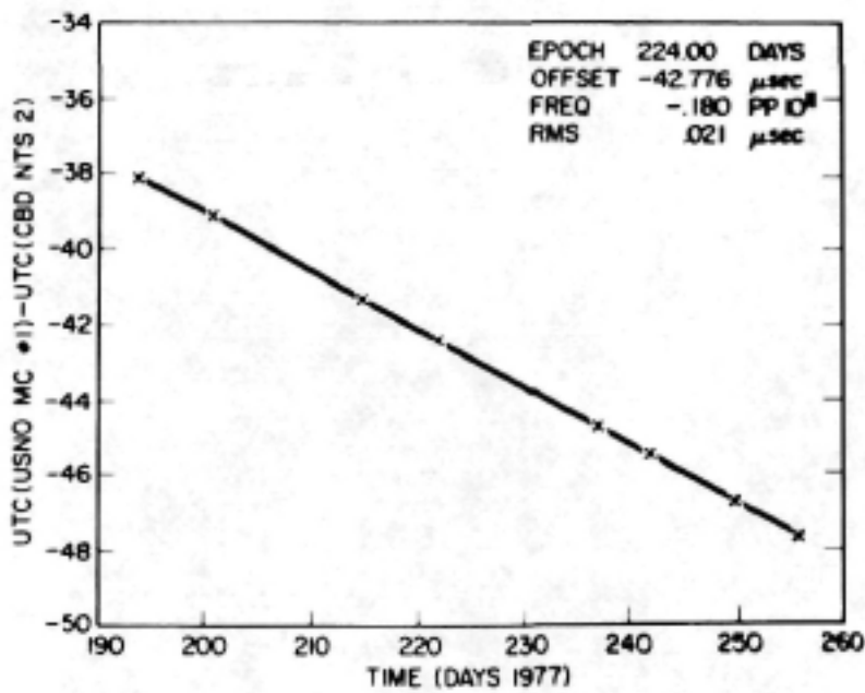
Fig. 22 - Frequency, USNO-CBD
