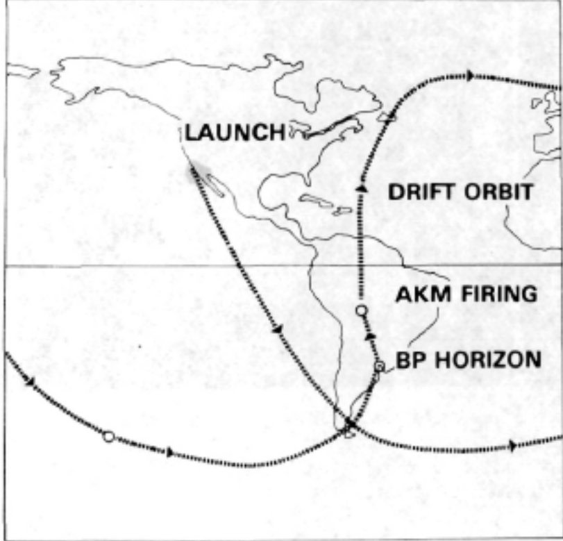
Fig. 4 - NTS-2 transfer orbit
