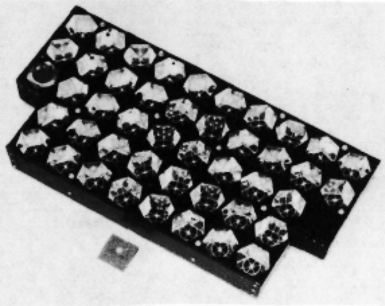
Fig. 35 - NTS-2 laser retroreflector
