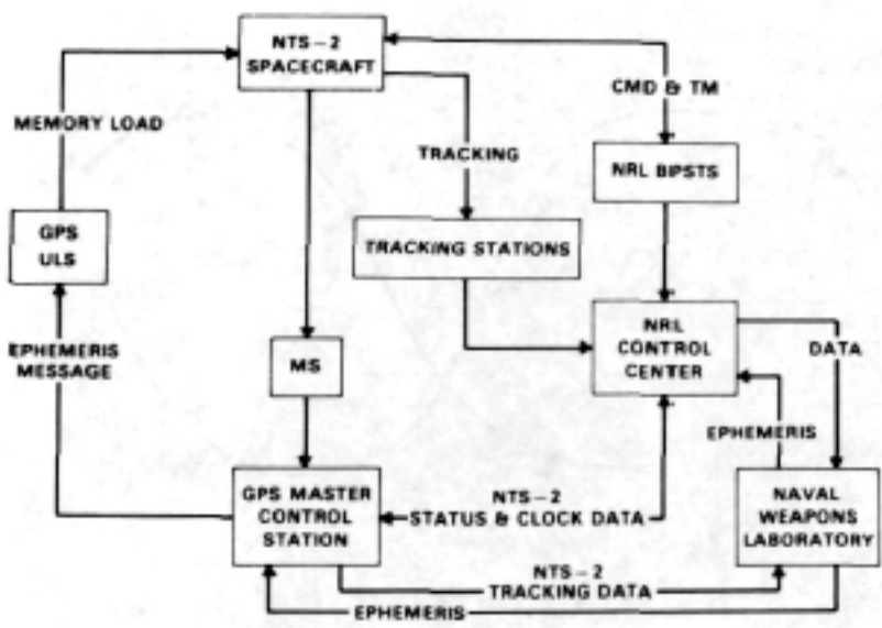
Fig. 7 - NTS-2 command and telemetry links
