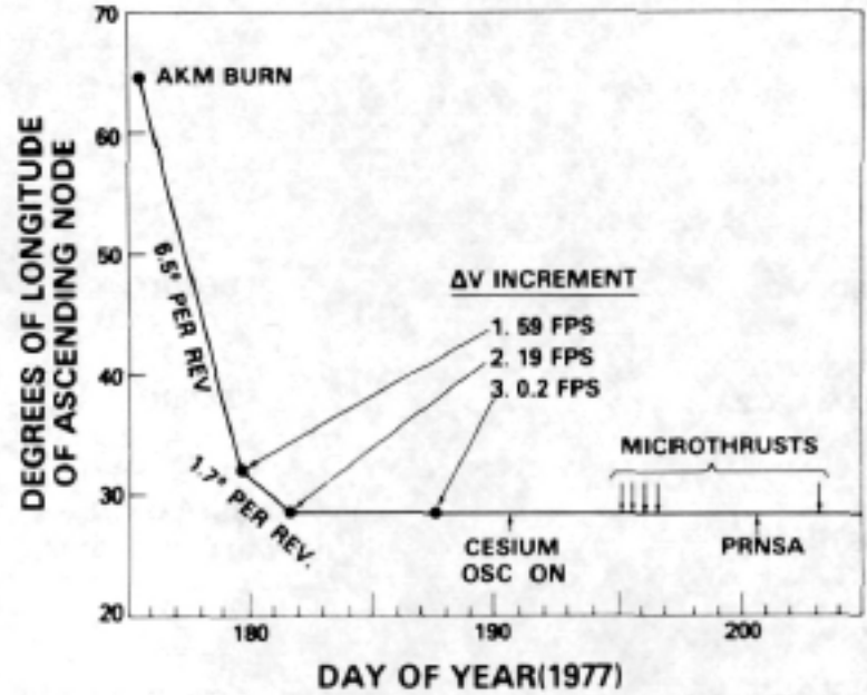
Fig. 9 - NTS-2 drift orbit adjustments
