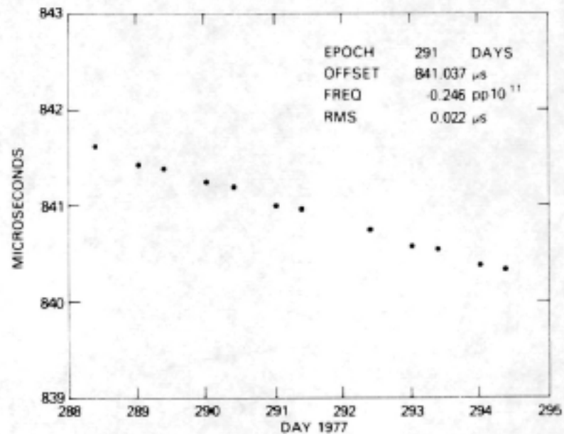
Fig. 25 - Frequency, NTS-CBD after C-field adjustment, 1977 day 287
